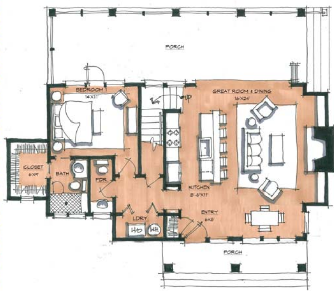
MAIN LEVEL FLOOR PLAN MAIN LEVEL SQ. FOOTAGE—1107 UPPER LEVEL SQ. FOOTAGE—343
